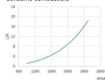
Consumo combustible
